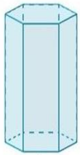
Prisma hexagonal
