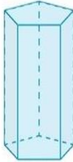
Prisma pentagonal
