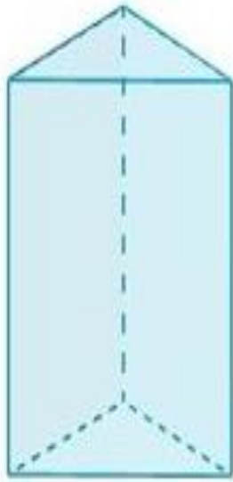
Prisma triangular
